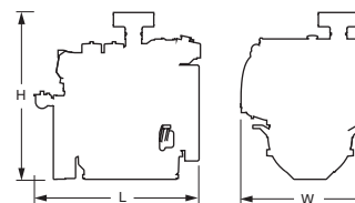
Naturally Aspirated
